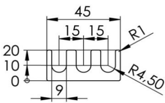
Shimblech
